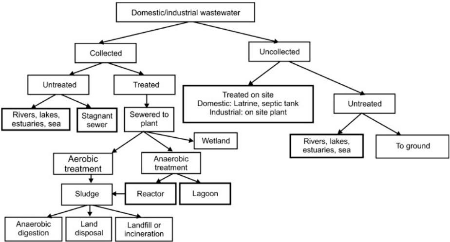
Figure 6 A typical flowchart of wastewater treatment process 1
