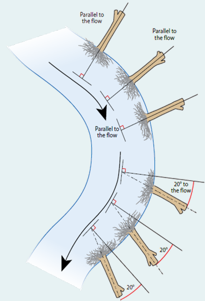
Plan showing position of root wads
